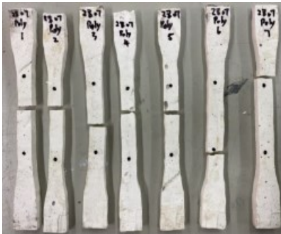
Dog-bone samples from tensile testing
