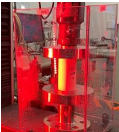
Uniaxial compressive strength testing
