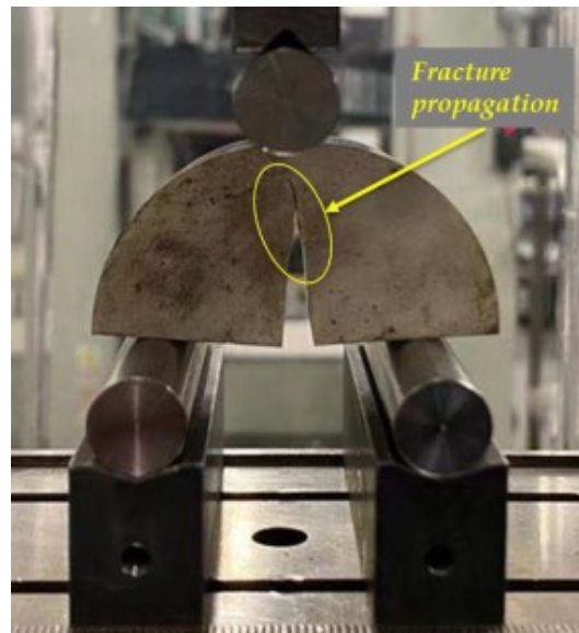
Fracture toughness test
